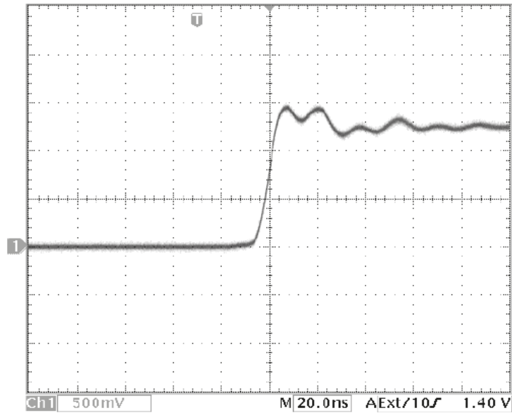
Figure 3 Rise Time
