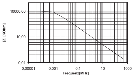
Typical input impedance PMT221A (switched to 10:1)
