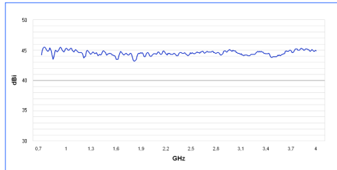
Diagramme de gain HyperLOG 7040X
