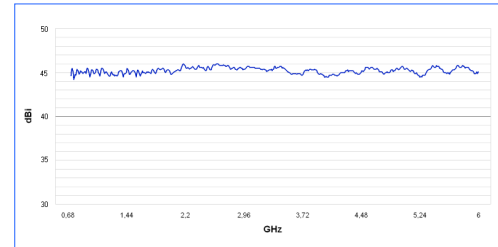
Diagramme de gain HyperLOG 7060X
