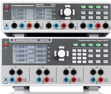
R&S® HMP2030 three-channel and R&S® HMP4040 four-channel power supply
