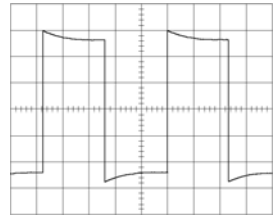
OVER COMPENSATED
