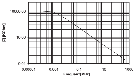
Typical input impedance PMS221A (switched to 10:1)
