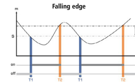
Measurement (m) < Threshold (S) during the time-delay T1: Alarm activation. Measurement (m) > Threshold (S) + Hysteresis (H) during time-delay T2: Alarm deactivation.
