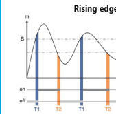
Measurement (m) > Threshold (S) during the time-delay T1: Alarm activation. Measurement (m) < Threshold (S) - Hysteresis (H) during the time-delay T2: Alarm deactivation.
